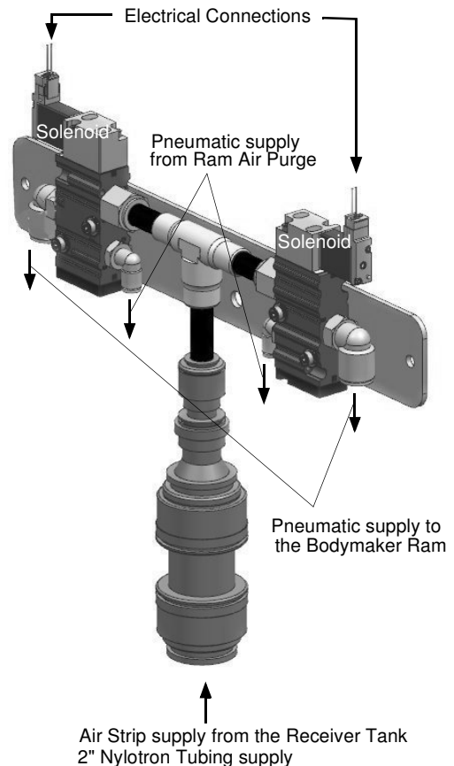
New Dual Air Strip Valve Assembly
