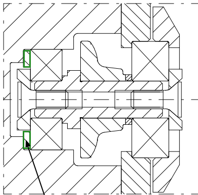
Waved Washer Part Number 27576213
