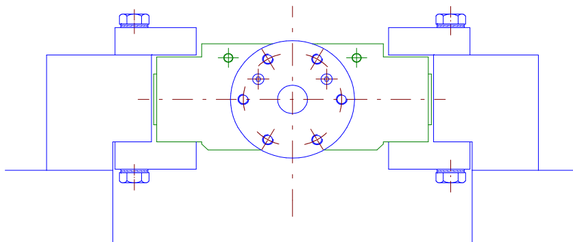
New Yoke Slide Assembly (Without bronze running pads)
