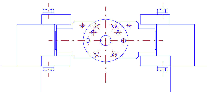
Old Yoke Slide Assembly (With bronze running pads)
