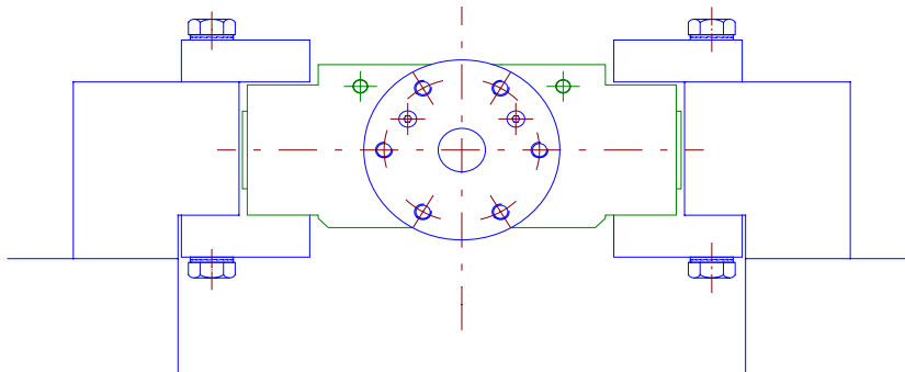
New Yoke Slide Assembly (Without bronze running pads)
