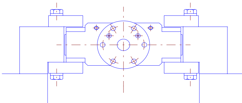
Old Yoke Slide Assembly (With bronze running pads)
